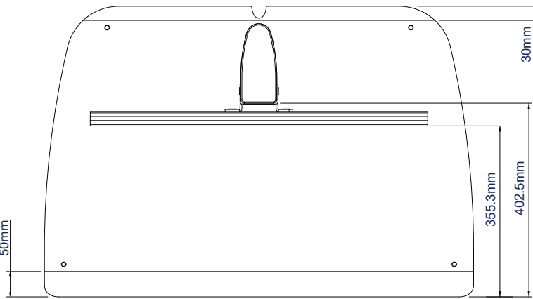
TOP VIEW WITH BT8380, BT8380-JPK & BT8390-050
